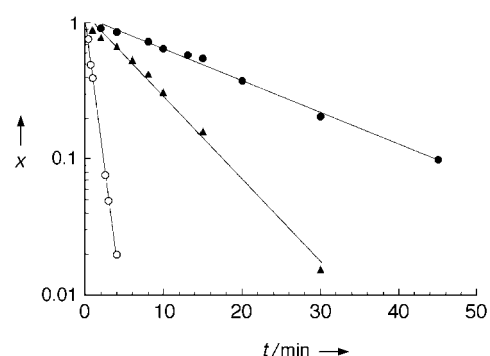
Figure 2. Kinetic data for the conversion of the native Ag upd layer to its halide-derivatized state for various contact times with 0.5 (●), 1.0 (▲), and 10 (○) \mu\text{M} KCl(aq) test solutions. The three data sets exhibit a first-order decay in the fractional intensity of the unconverted Ag(upd)/Au(111) signal ( x ), and the rates of conversion across these data sets vary linearly with their halide concentration.
